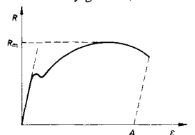
Dijagram R, \epsilon
